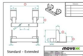
Customized Hook (EXTENDED)
