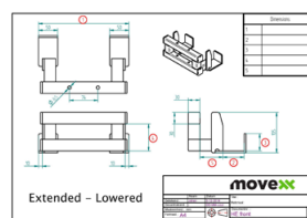
Customized Hook (EXTENDED / LOWERED)
