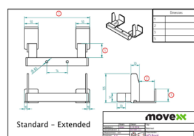
Customized Hook (EXTENDED)
